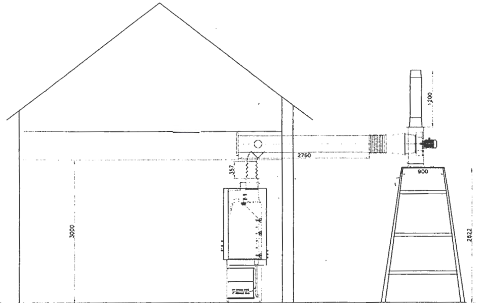
SIDE VIEW 4' ABP Benchtop FH MS Stand For Blower will be in client's scope
