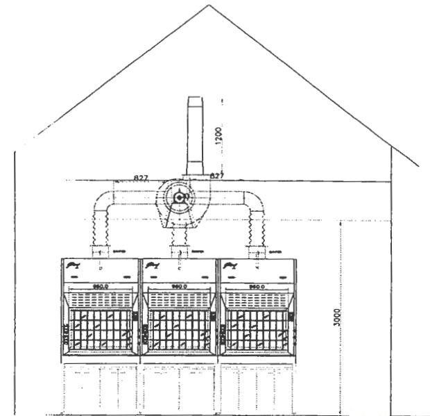
4' ABP Benchtop FH FRONT VIEW
